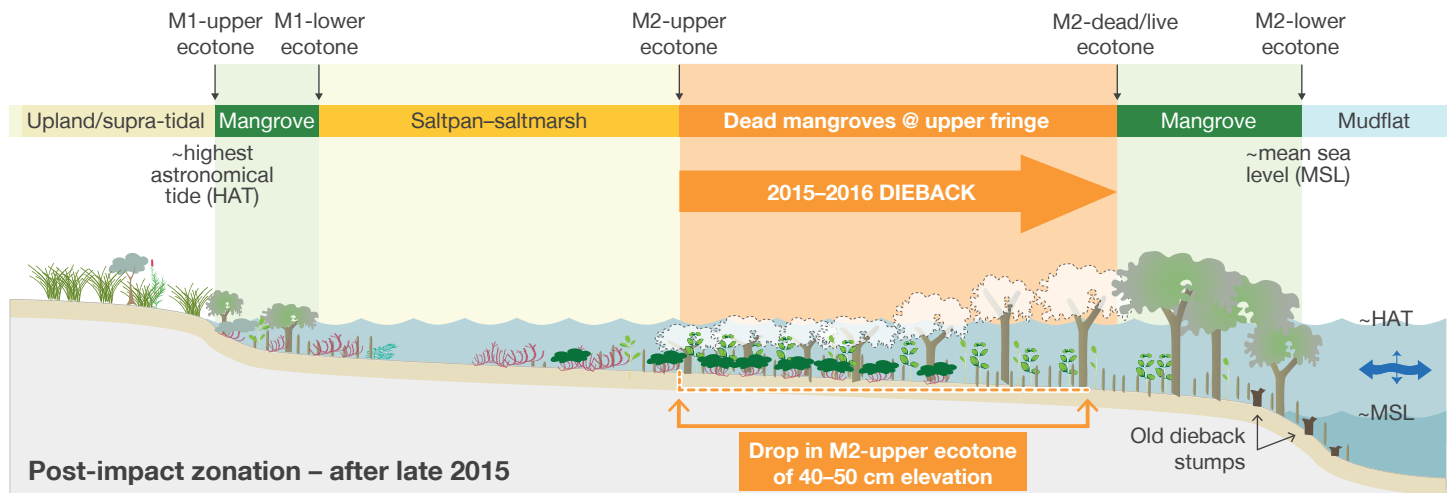
This diagram depicts characteristics used in the field studies to define elevations and distances along transects as vegetation ecotones along the upper half of the tidal range – the niche of the tidal wetland zone. The profile images depict a typical Gulf of Carpentaria shoreline, before and after the severe impact of the 2015–2016 dieback of the seaward mangrove fringe. Mangroves at the upper edge of the mangrove zone (M2-upper ecotone) died, shifting that ecotone 40–50 cm lower in elevation, to the M2-dead/live ecotone position.
